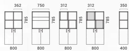
Shelving units for mounting on cabinets – ready-made configurations
