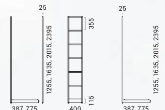
Shelving units – modular configurations
