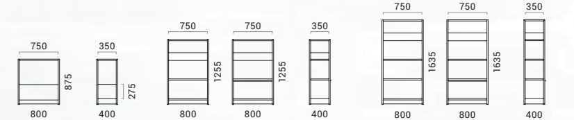
Planter shelf units – ready-made configurations
